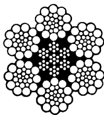
6 x 26 Warrington Seale IWRC
