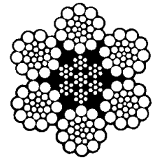
6 x 26 Warrington Seale IWRC
