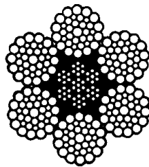
6 x 36 Warrington Seale IWRC
