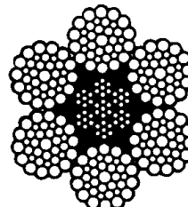
6 x 36 Warrington Seale IWRC
